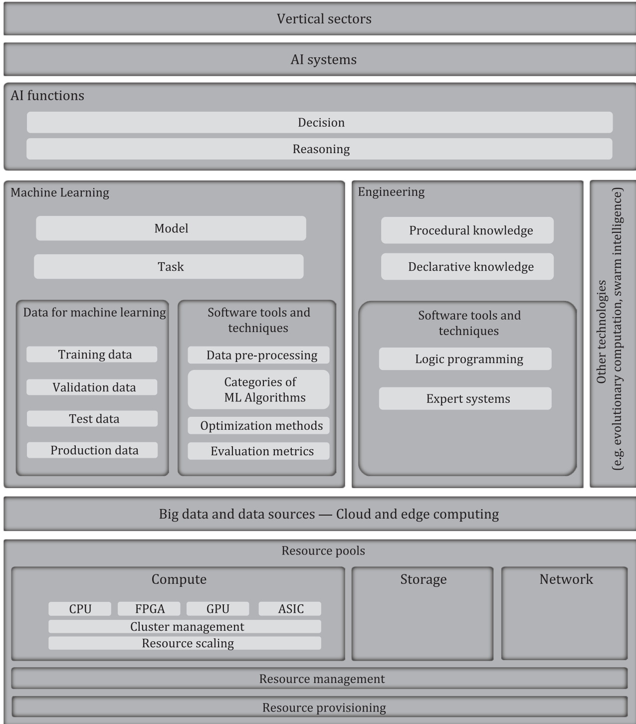
Figure 6 — AI ecosystem
